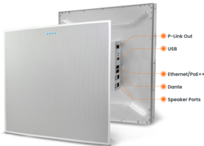
BMA 360DX All-in-One Innovative Ceiling Tile (Photo: Business Wire)
